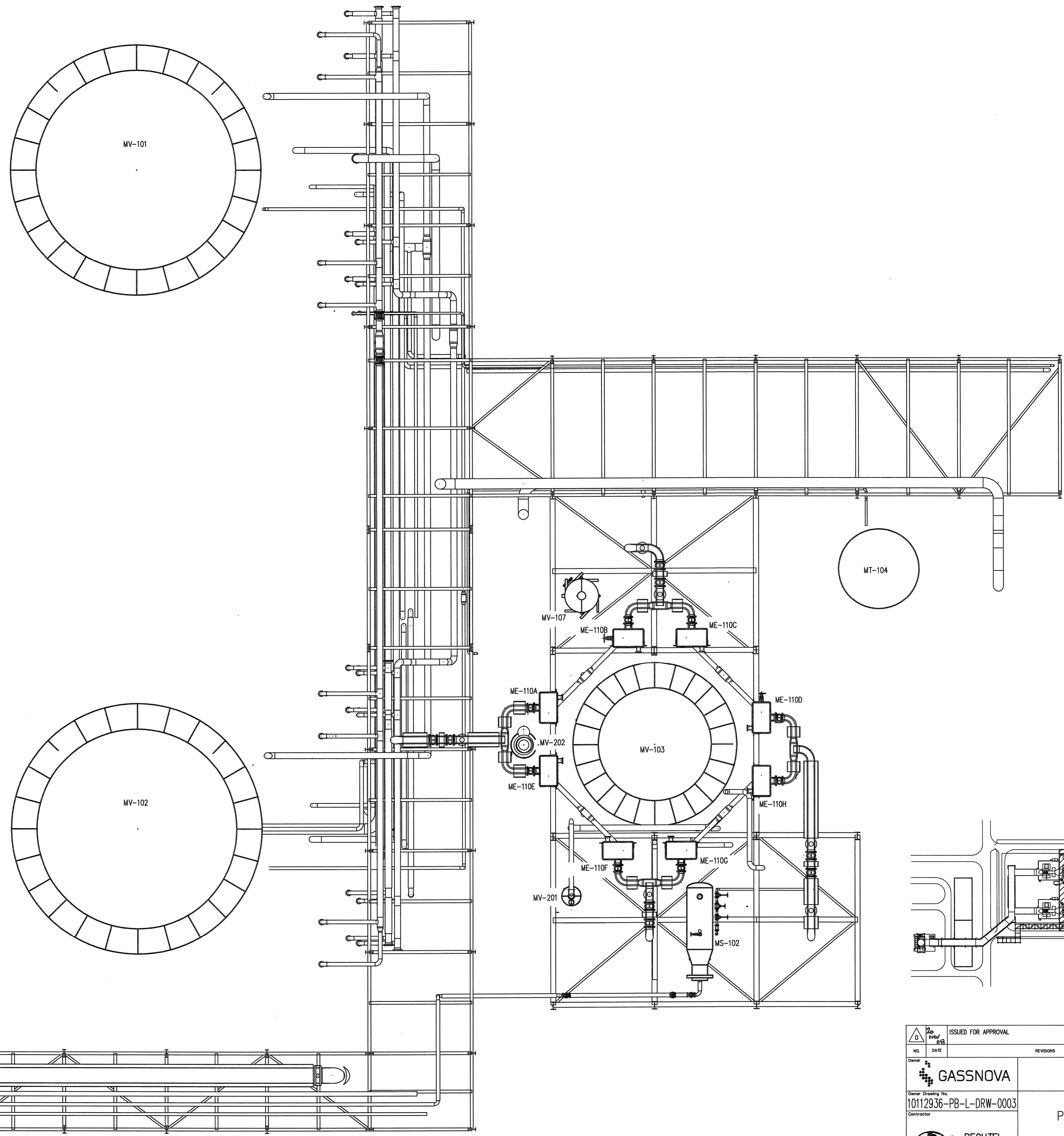
PLAN VIEW @ EL. +16.95M
