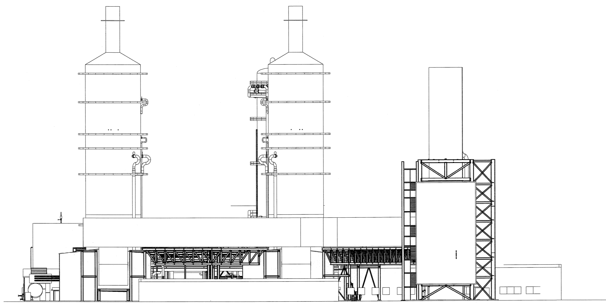
COMPOSITE MODEL END VIEW LOOKING EAST FROM NATURKRAFT FACILITY
